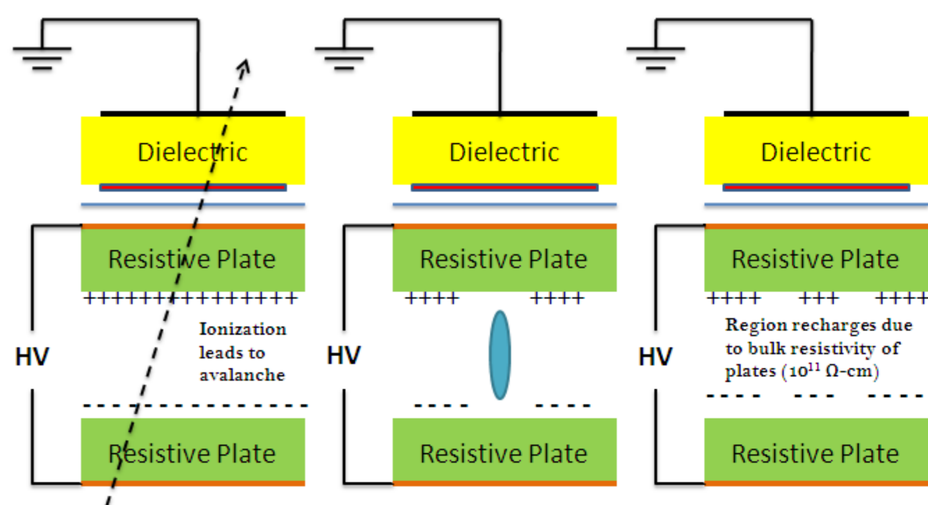
Figure: Principle of operation of a RPC.
